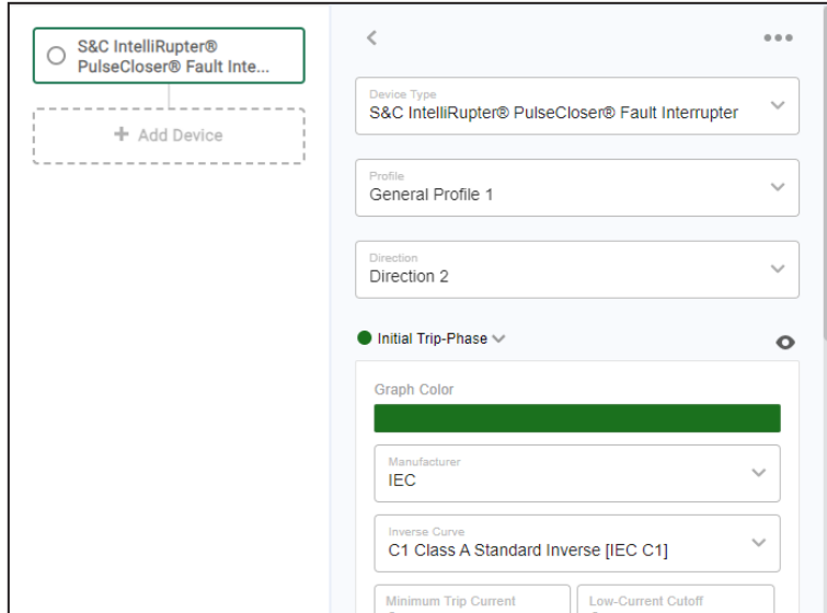
Figure 12. The device parameters for an IntelliRupter fault interrupter.
