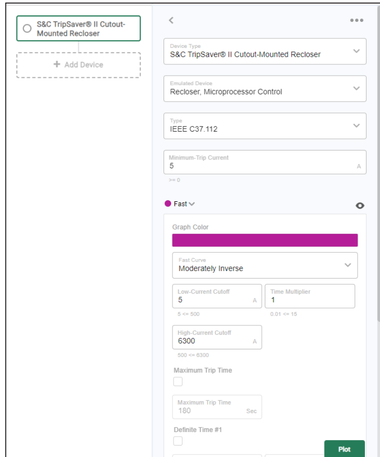
Figure 19. The Fast curve configuration settings.
