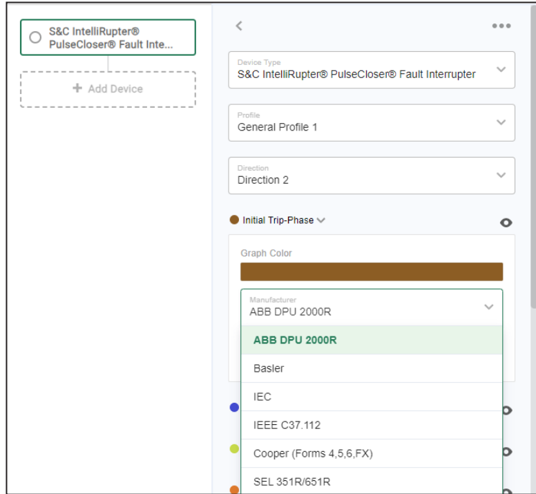
Figure 14. The device selection for an Initial Trip-Phase TCC curve.
