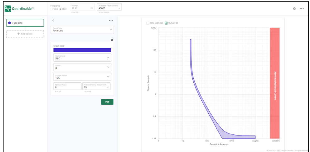
Figure 6. The TCC curve generated by the Plot button.
